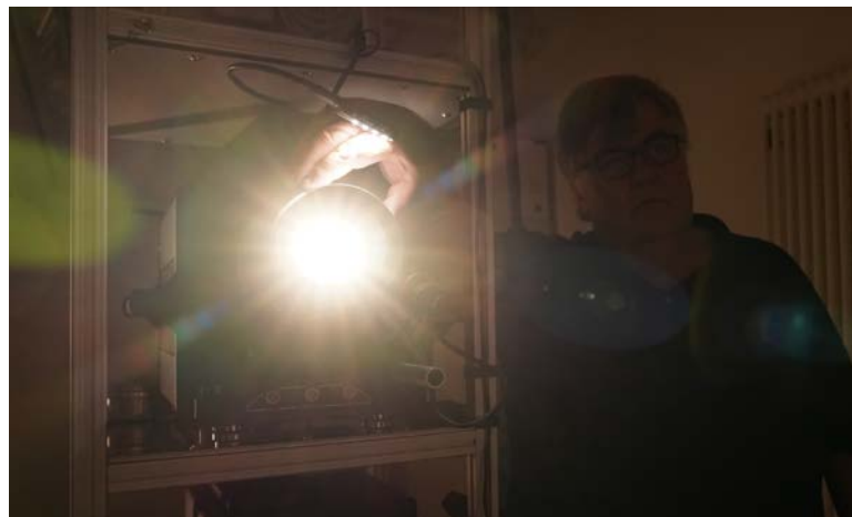
Christian Agerer “driving” the custom-designed Trioptics MTF optical testing device. As mentioned, each ARRI Rental facility in Munich, Berlin, London, Burbank and New York has commissioned one of these. ARRI Cine Technik also uses this machine in manufacturing and QC of Signature Primes. In this photo taken with an ARRI DNA LF 35mm at T2, note how the extremely tuned field curvature blurs and distorts the keyboard, above at right.
