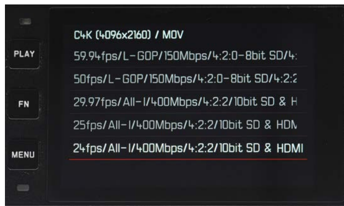
10. Select C4K (4096x2160), jog right to: 24 fps / All-I / 400 Mbps / 4:2:2 / 10-bit / SD & HDMI (Record to internal SD card or externally via HDMI).
