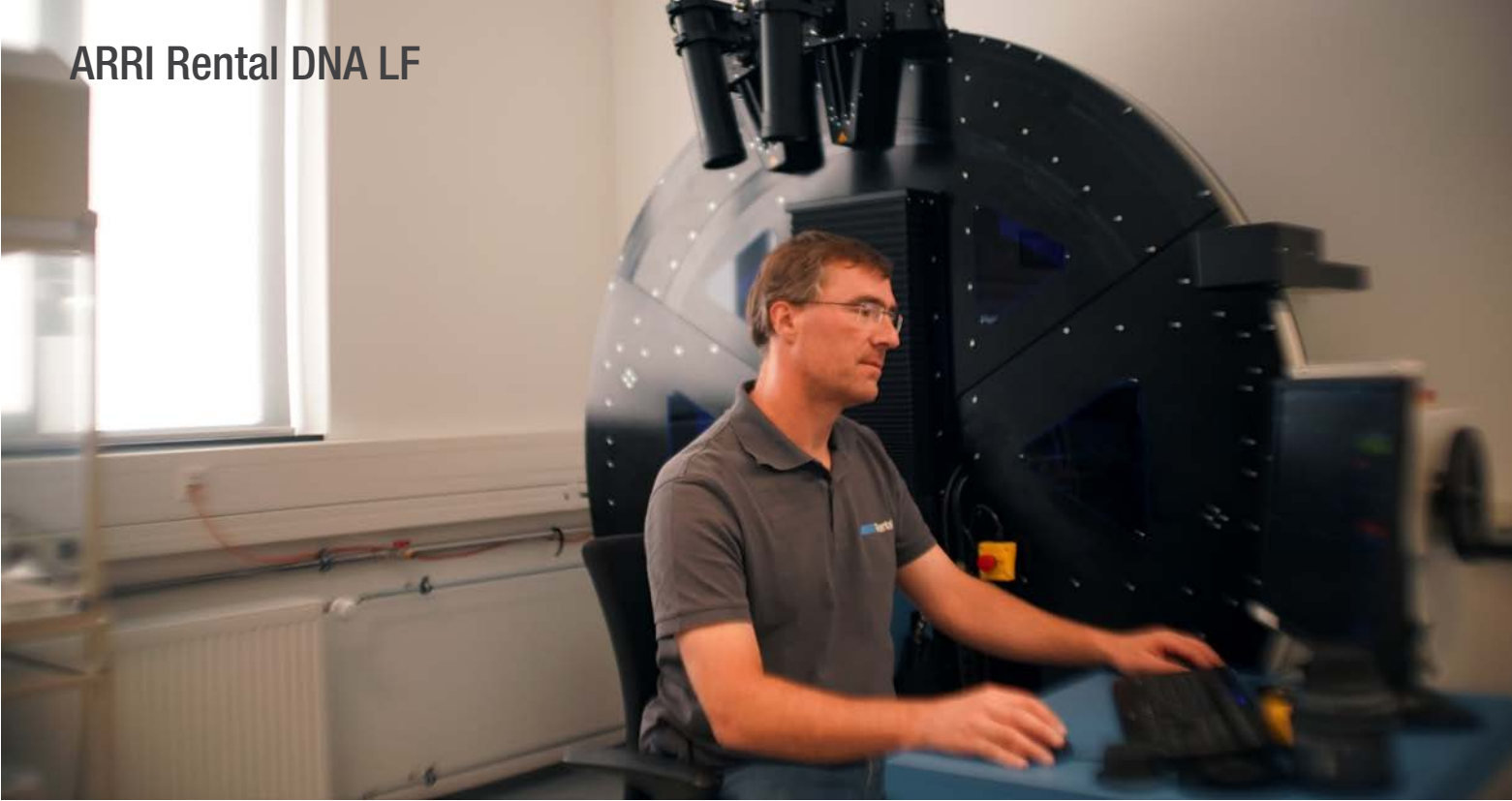
Christian Agerer “driving” the custom-designed Trioptics MTF optical testing device. As mentioned, each ARRI Rental facility in Munich, Berlin, London, Burbank and New York has commissioned one of these. ARRI Cine Technik also uses this machine in manufacturing and QC of Signature Primes. In this photo taken with an ARRI DNA LF 35mm at T2, note how the extremely tuned field curvature blurs and distorts the keyboard, above at right.
